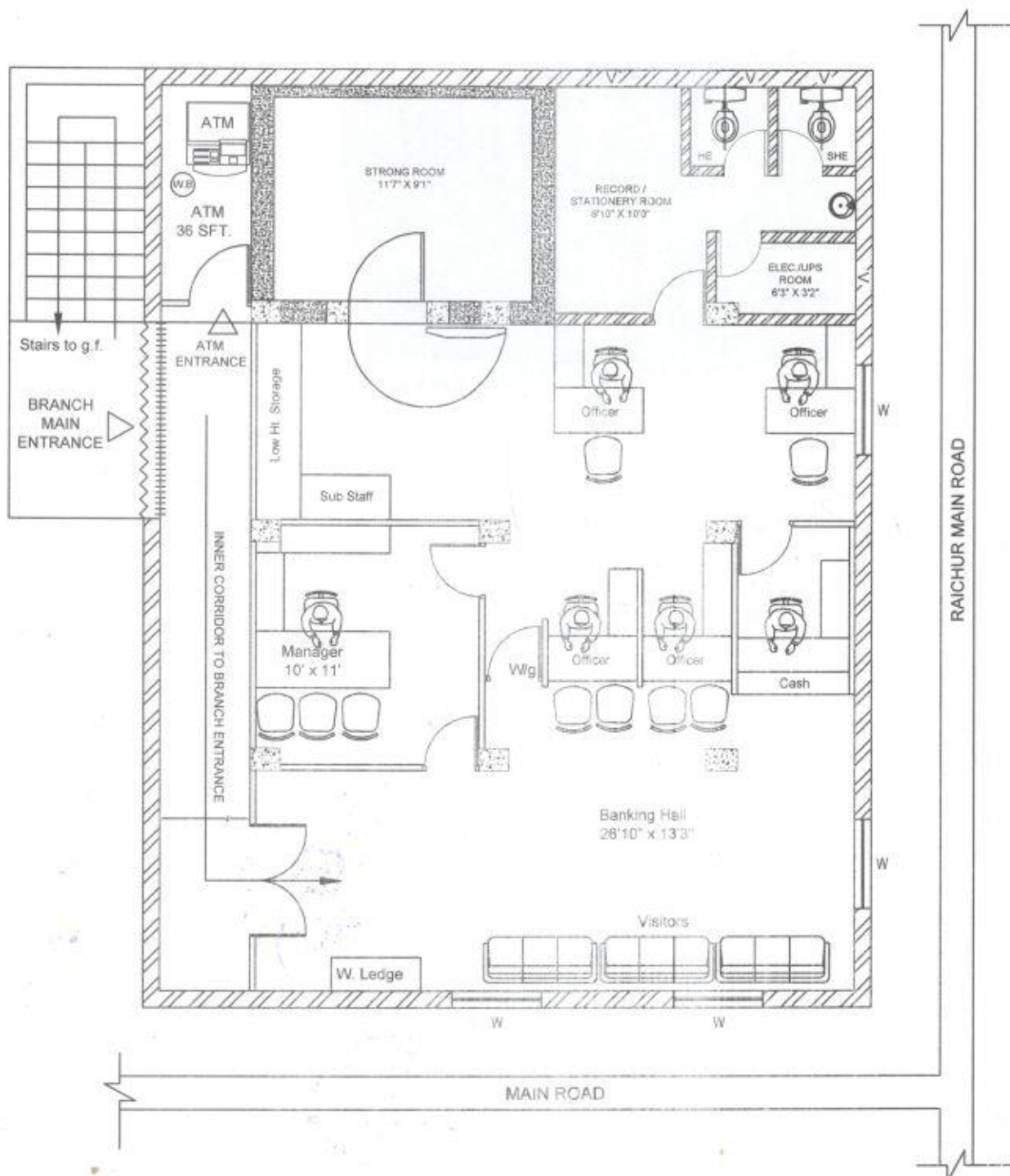
PROPOSED INTERIOR LAYOUT FOR UCO BANK, MARIKAL BRANCH - 1ST FLOOR
