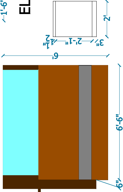
ELEVATION D
