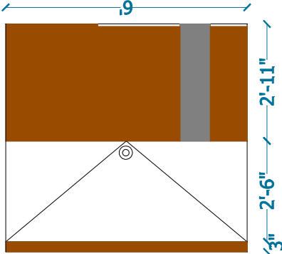
ELEVATION C
