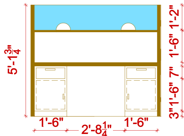
SIDE B
