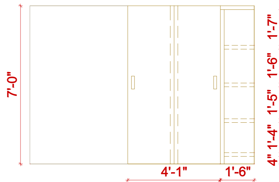
ELEVATION C
