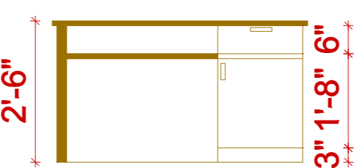
SIDE B
