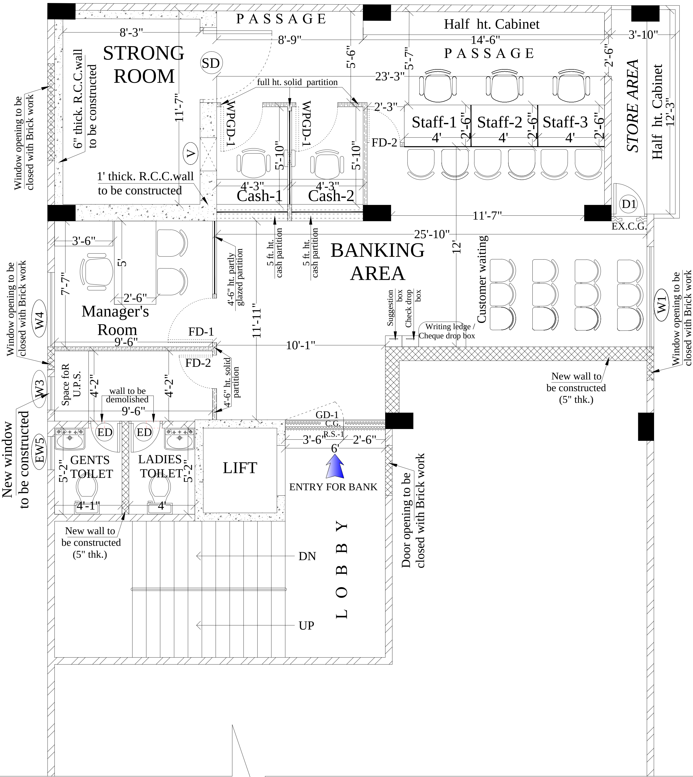
PROPOSED LAYOUT (FIRST FLOOR)
