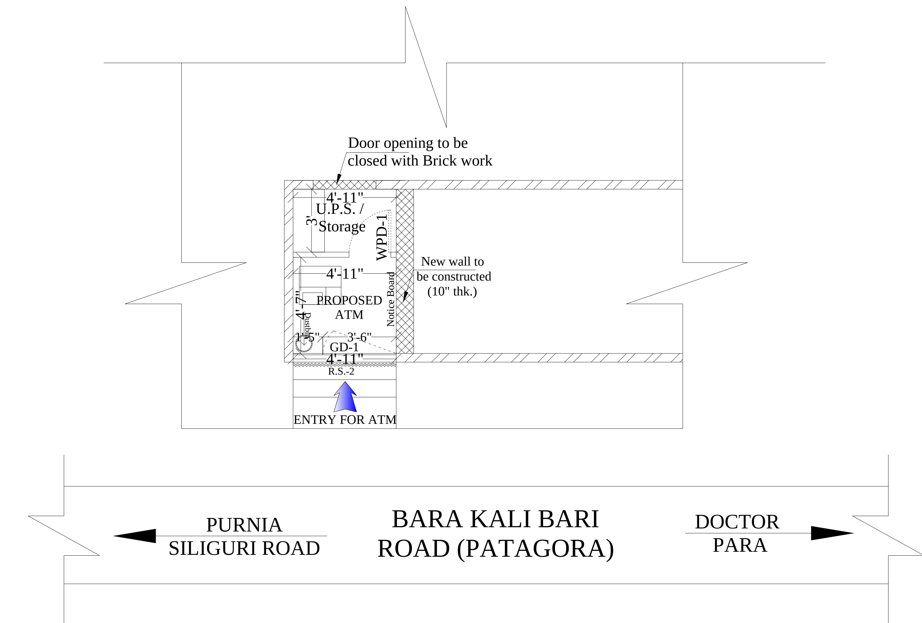
PROPOSED LAYOUT (GROUND FLOOR)
