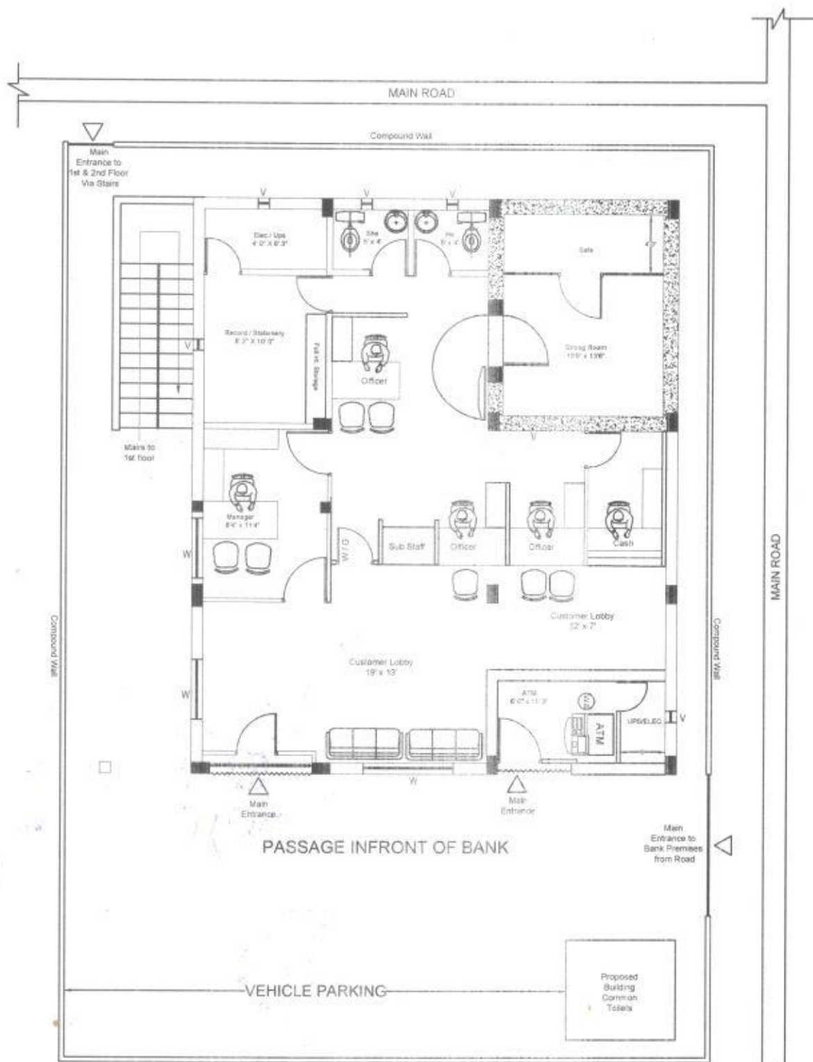
TULLUR BRANCH - PROPOSED CIVIL & INTERIOR LAYOUT - Rev.OPTION -2
